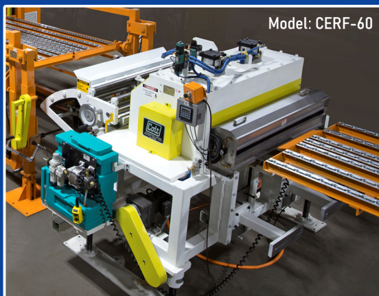
Heavy-Duty Feeder w/ Material Strip Support
